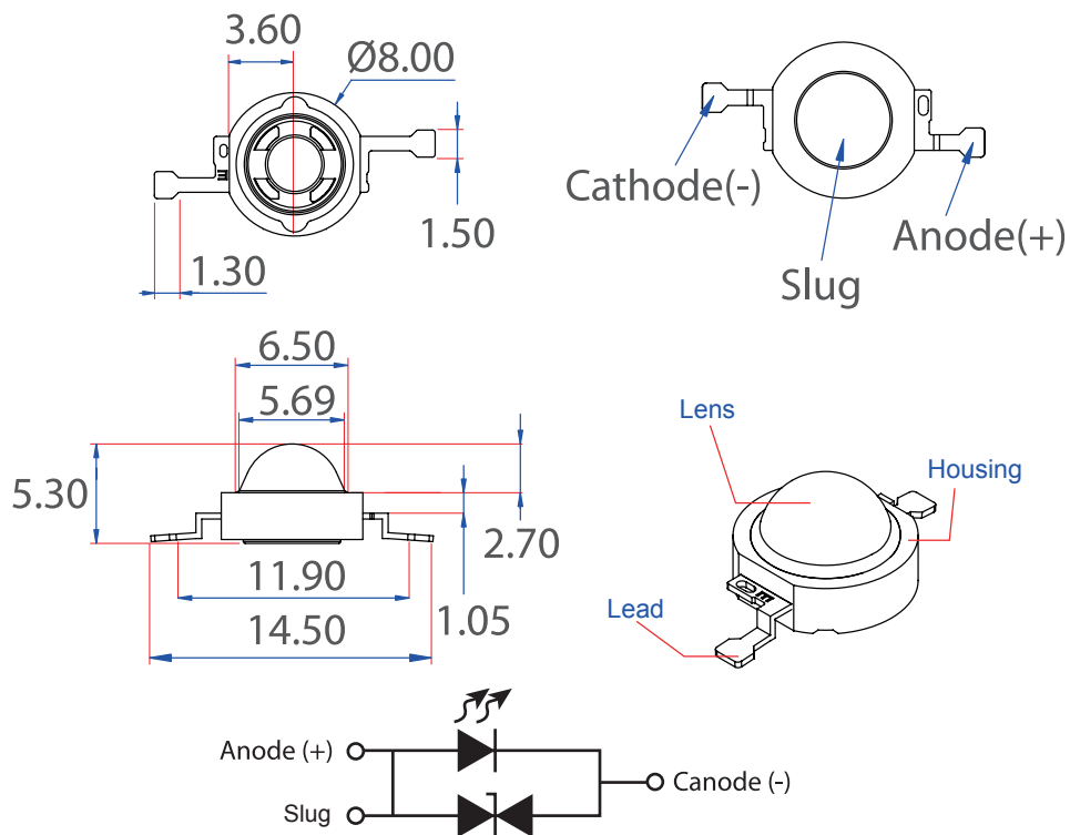
Figure 1. Edixeon® S series dimensions
