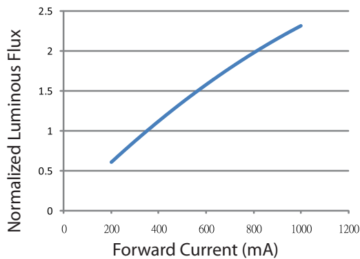
Figure 8. Relative luminous flux vs. forward current for Cool White
