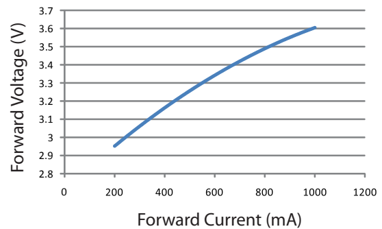
Figure 7. Forward voltage vs. forward current for Cool White, Neutral White and Warm White
