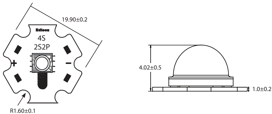
Figure 2. Federal 5050 Series Star PCB type Dimension
