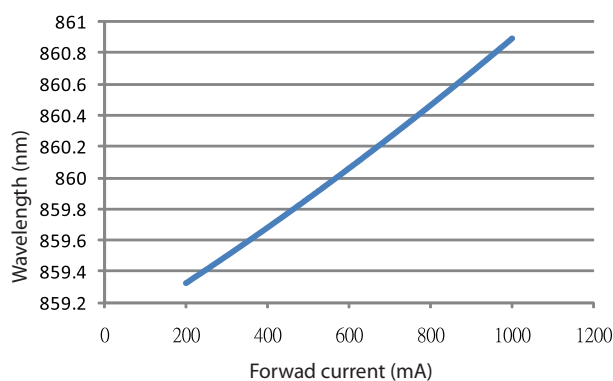
Figure 14. Wavelength vs. forward current for Federal 3535 IR850
