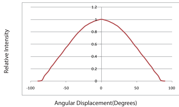
Figure 6. Emission Angle for Federal 3535 IR850
