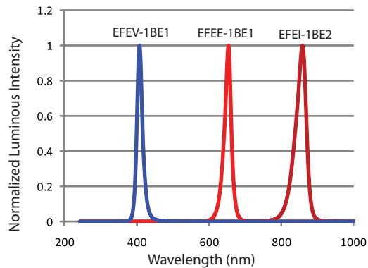
Figure 5. Color Spectrum at T_j=25\text{ }^{\circ}\text{C}
