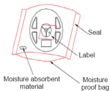
Figure 21. Federal 3535 Package
