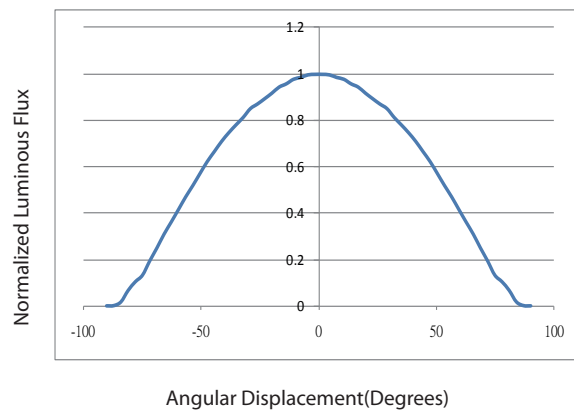
Figure 7. Emission Angle for Federal 3535 UV
