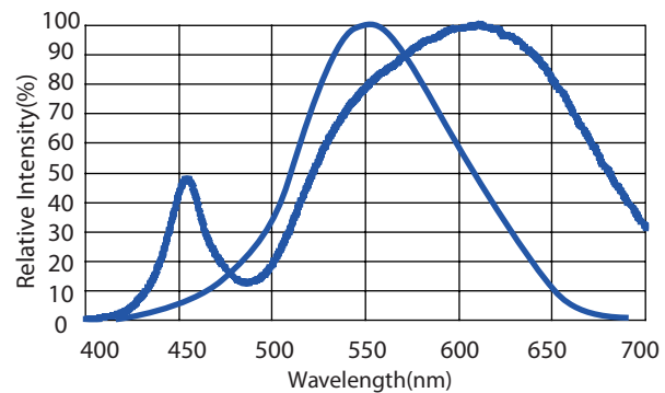
Figure 6. Color Spectrum for Warm White at T_j=25^\circ\text{C} .
