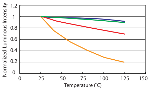
Figure 9. Relative luminous flux vs. junction temperature for True Green, Blue, Red and Amber.
