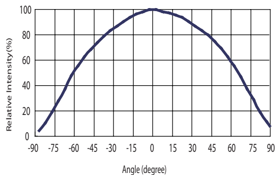
Figure 7. Emission Angle
