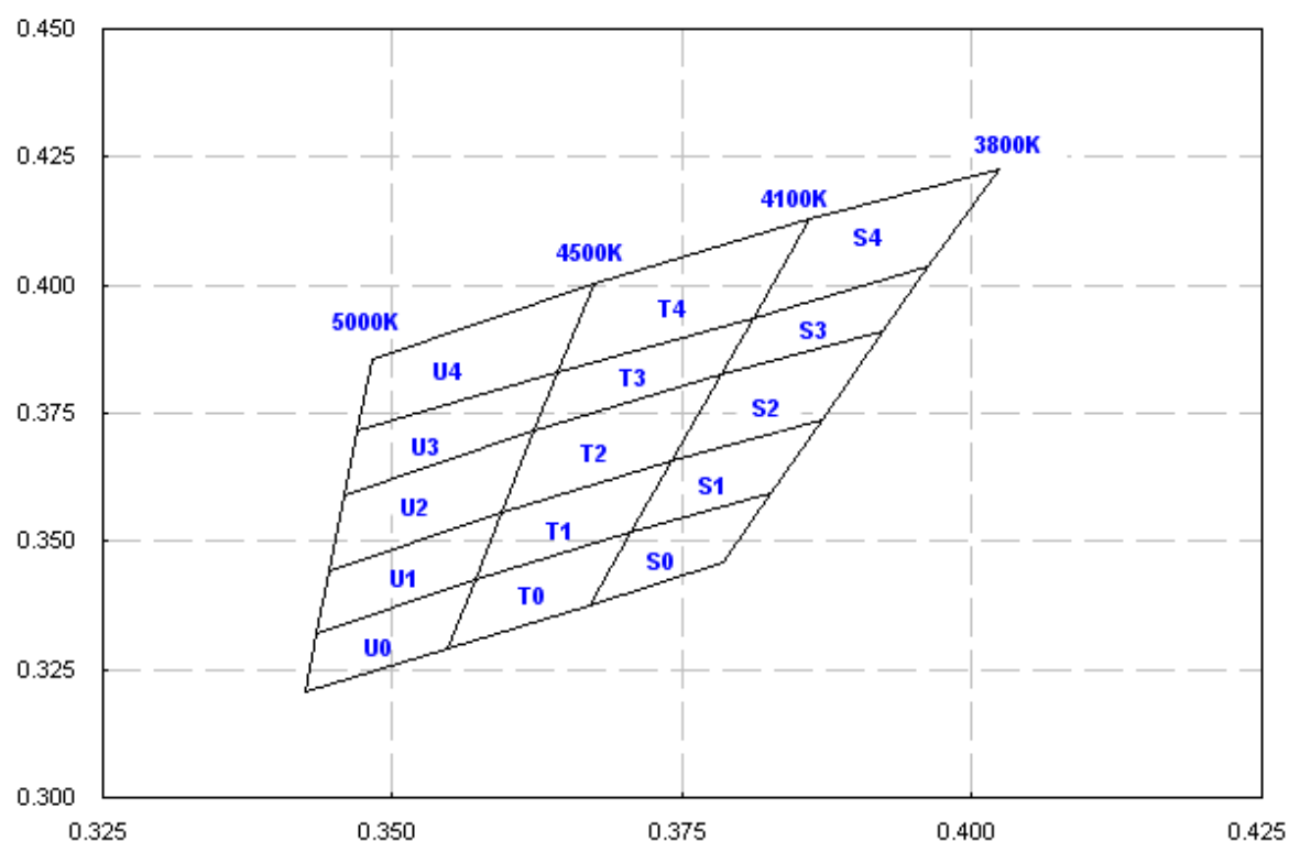
< Figure 14 PLCC 3528 series chromaticity diagram >
