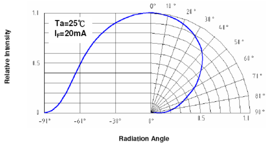
<Figure 3. Beam pattern diagram for PLCC 3528 series >
