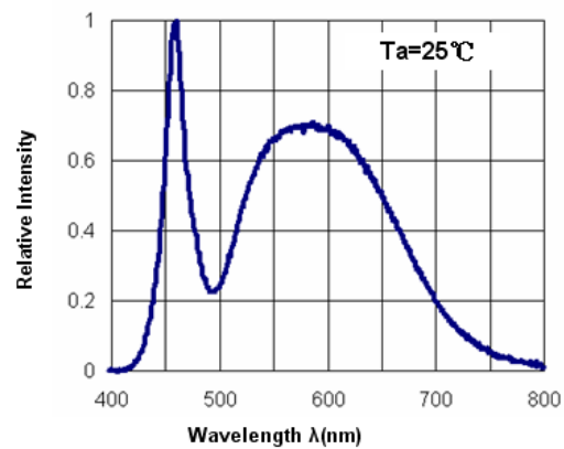
< Figure 4 Wavelength & relative intensity for PLCC 3528 series.>
