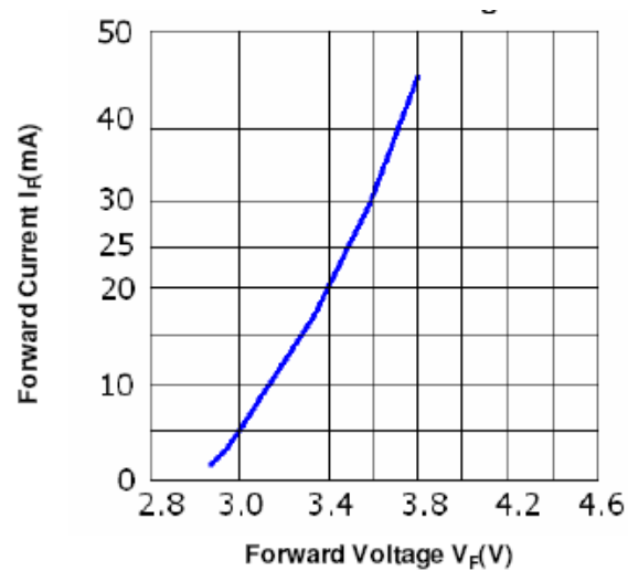
< Figure 8 Forward voltage & forward current for PLCC 3528 series >
