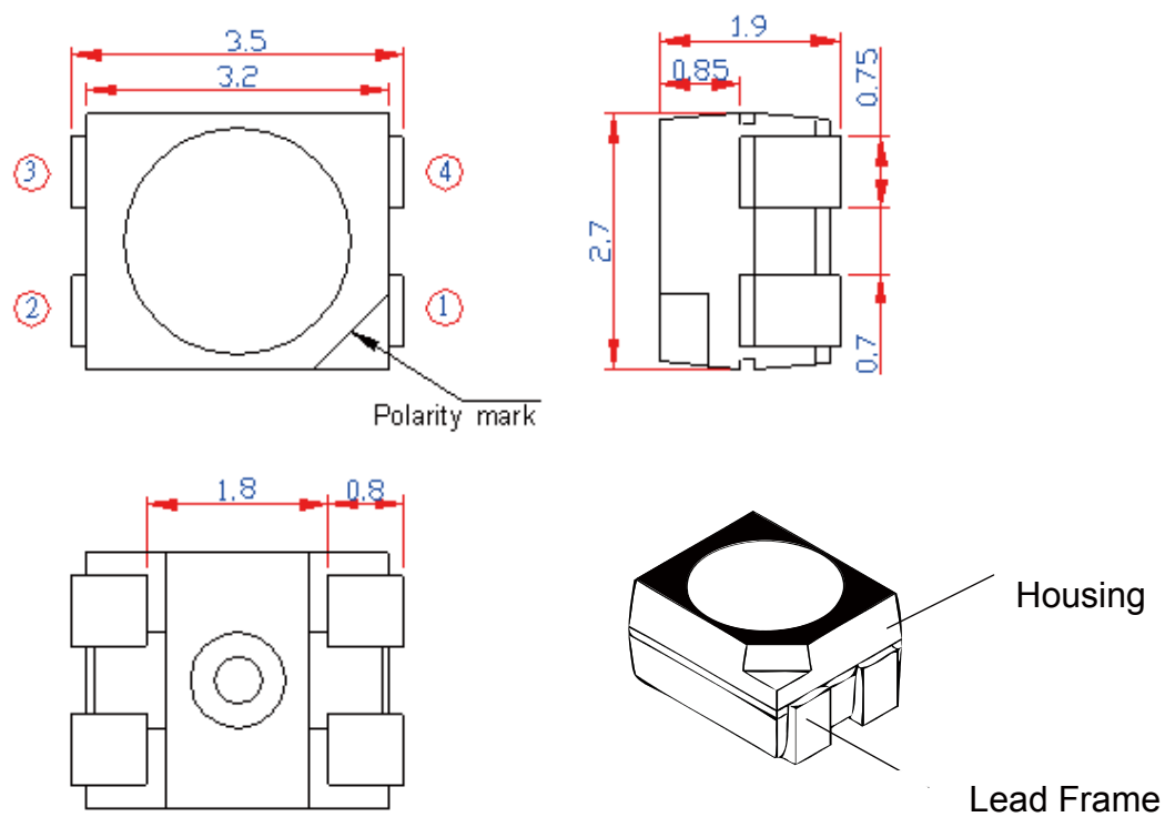
Figure 2. PLCC 3528 series Dimension
