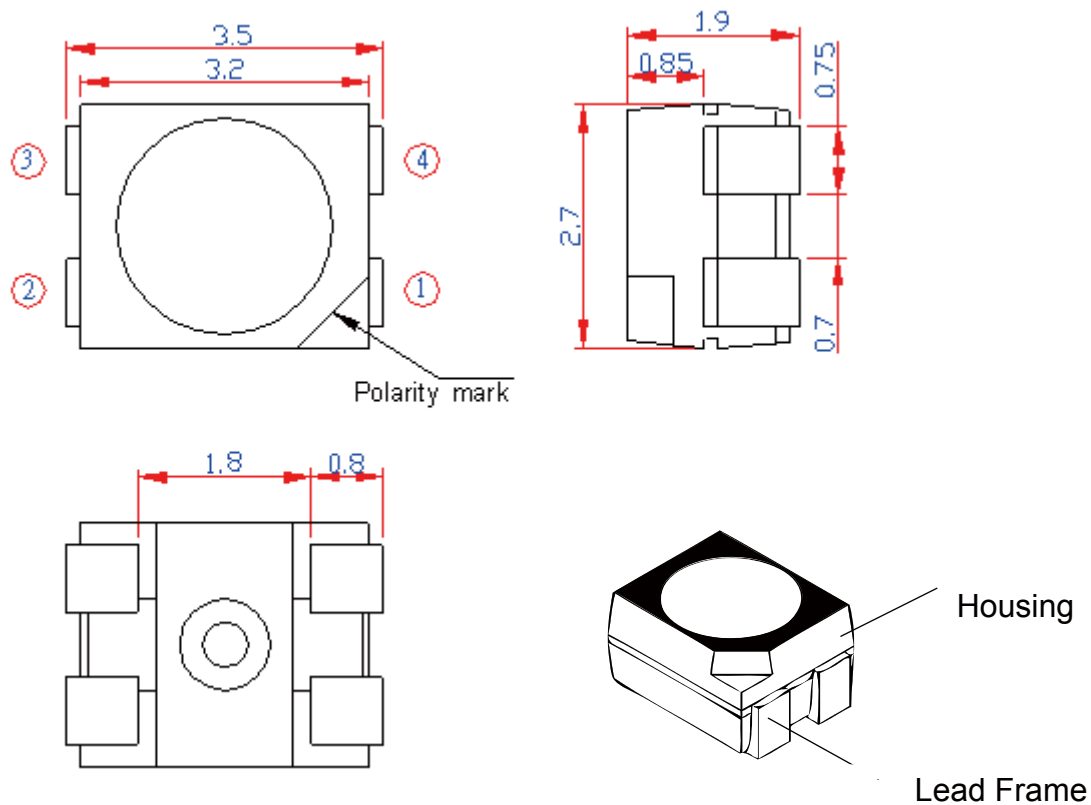
Figure 2. PLCC 3528 series Dimension
