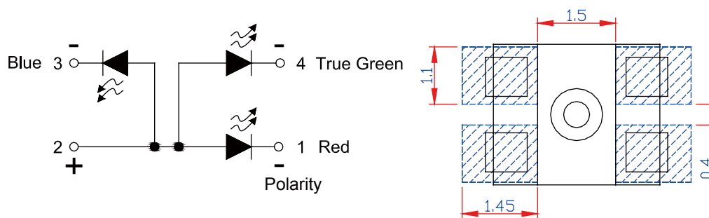
Figure 2. PLCC 3528 series Dimension
