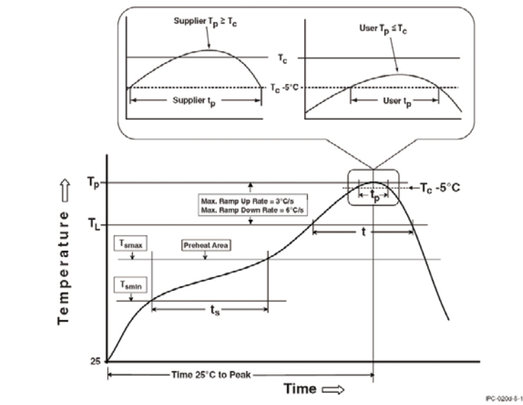
Figure 9 . Reflow Profiles
