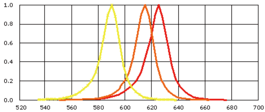
Figure 4. Wavelength & relative intensity for PLCC 3528 series
