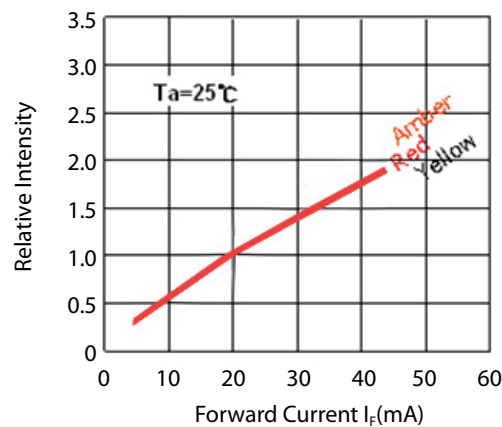
Figure 6. Forward current & relative intensity for PLCC 3528 series
