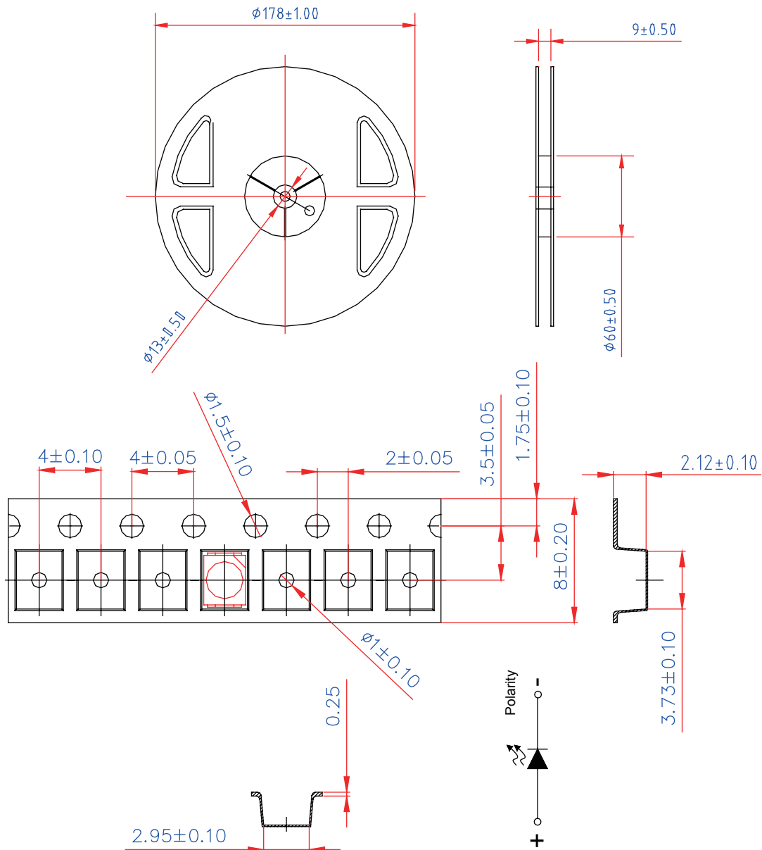
Figure 9. Taping reel dimensions
