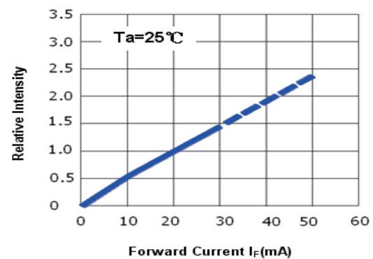
Figure 8. Forward current & relative intensity for PLCC 3528 series
