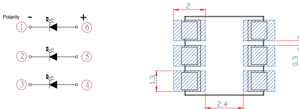
Figure 3. PLCC 5050 series circuit diagram
