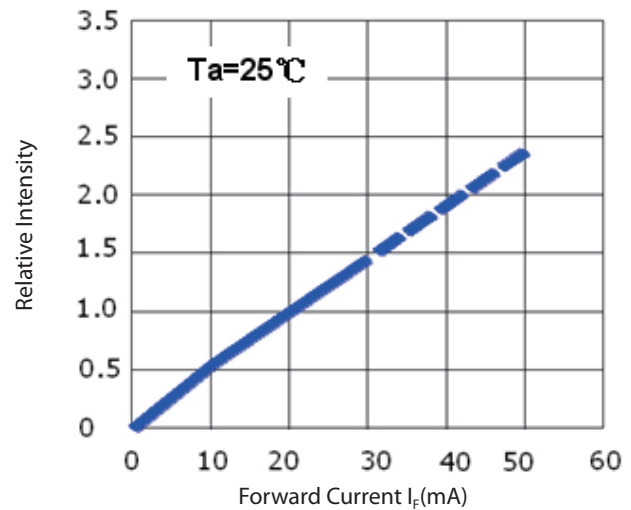
Figure 7. Forward current & relative intensity for PLCC 5050 series
