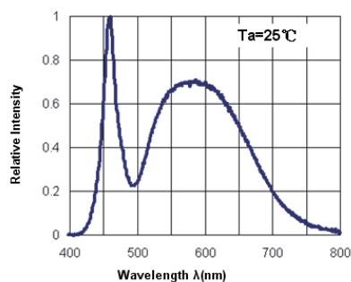
Figure 5: Wavelength & relative intensity for PLCC 5050 series
