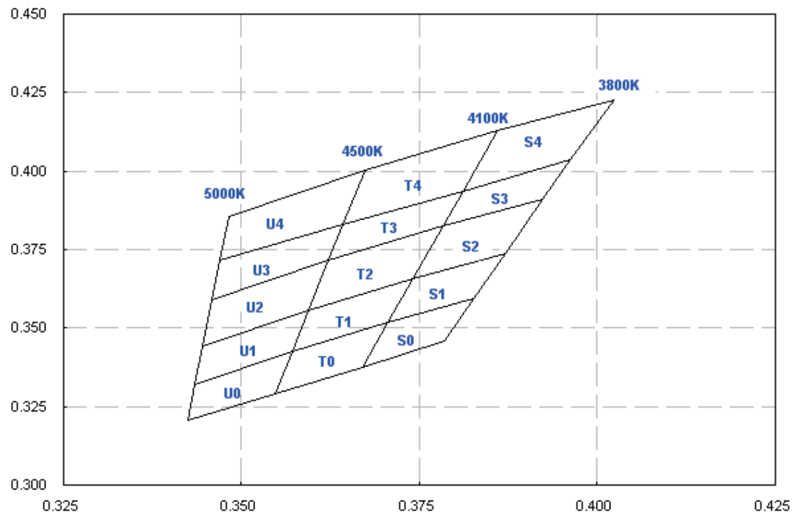
Figure 15. PLCC 5050 series chromaticity diagram
