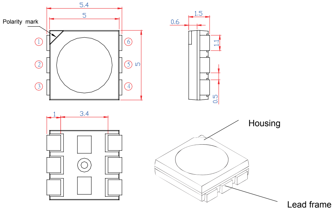
Figure 2. PLCC 5050 series Dimension
