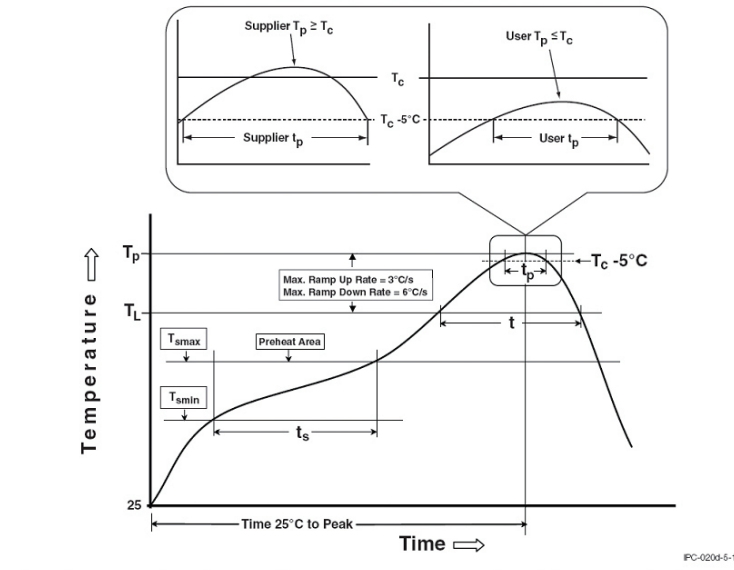
Figure 12. Reflow Profiles
