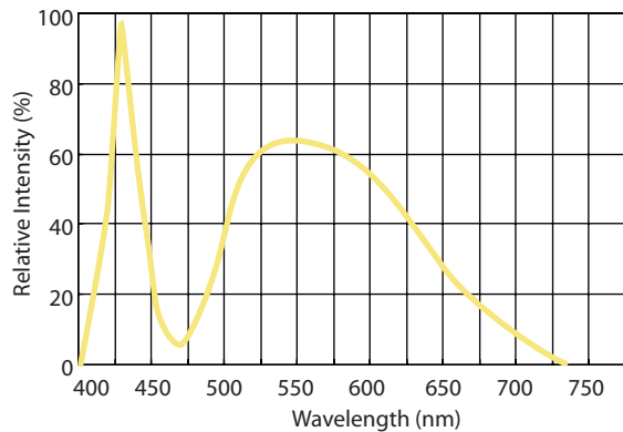
Figure 11. Color Spectrum for Neutral White at a typical CCT.
