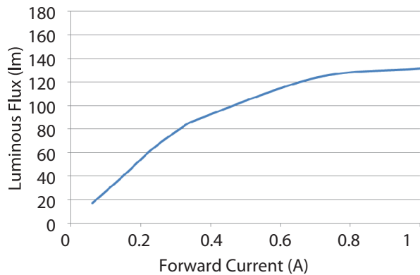
Figure 8. Forward current & relative luminous at T_a=25^\circ\text{C} for 1W PLCC
