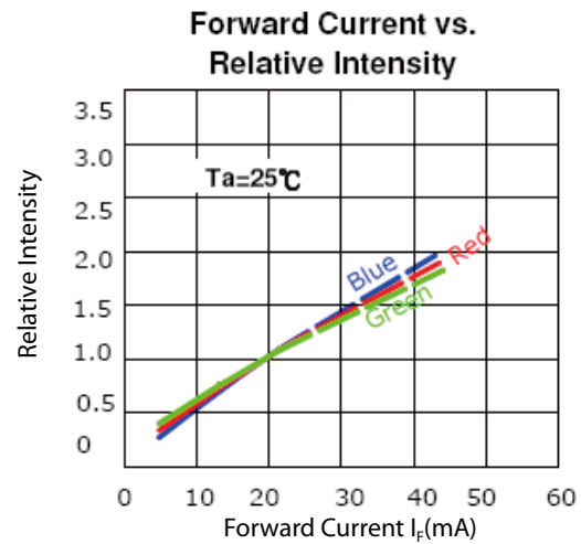
Figure 8. Forward current & relative intensity for PLCC 5050 series
