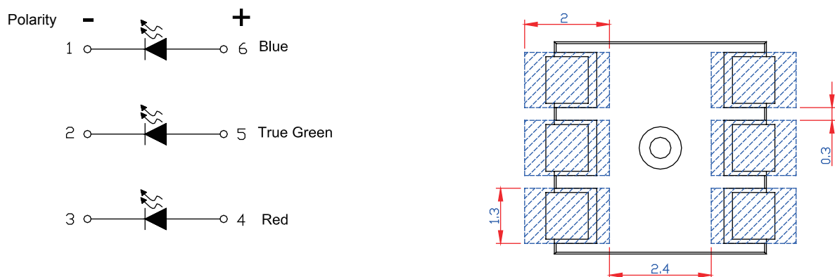
Figure 2. PLCC 5050 series circuit diagram and recommended soldering pad
