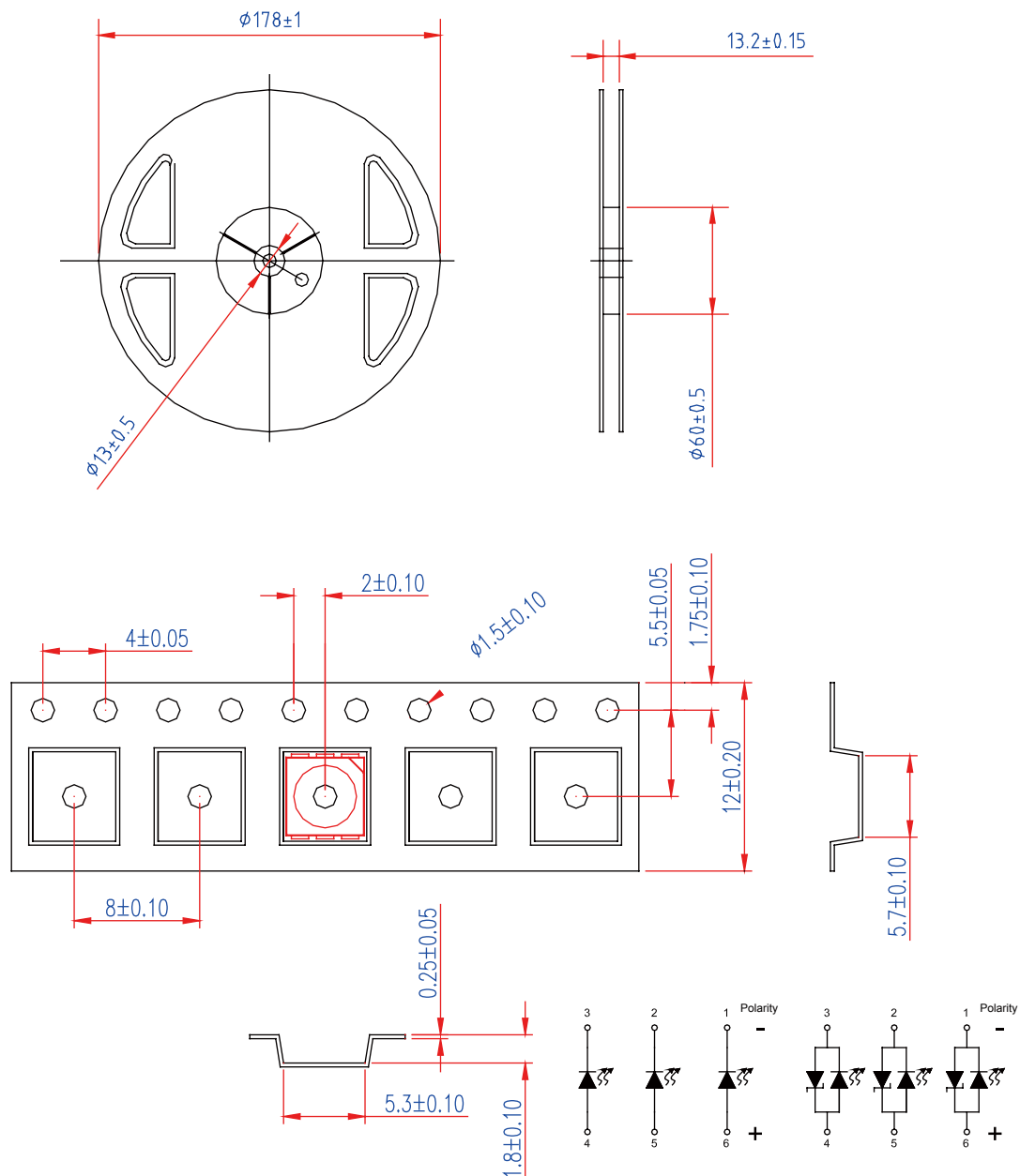
Figure 11. Taping reel dimensions
