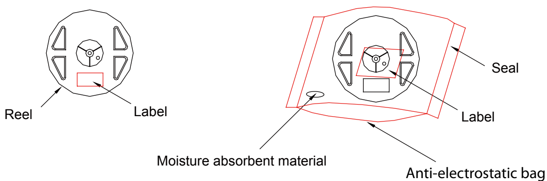
Figure 12. Packaging diagram
