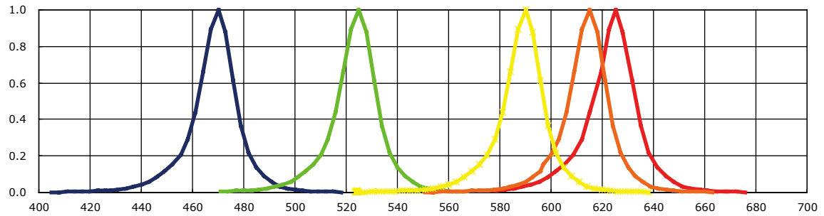
Figure 5. Wavelength & relative intensity for PLCC 5050 series
