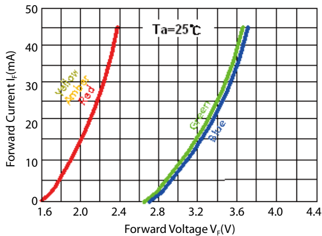
Figure 8. Forward voltage & forward current for PLCC 5050 series
