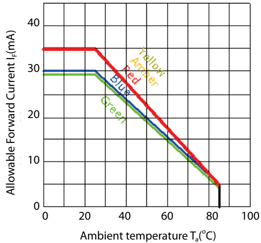
Figure 6. Ambient temperature & forward current for PLCC 5050 series
