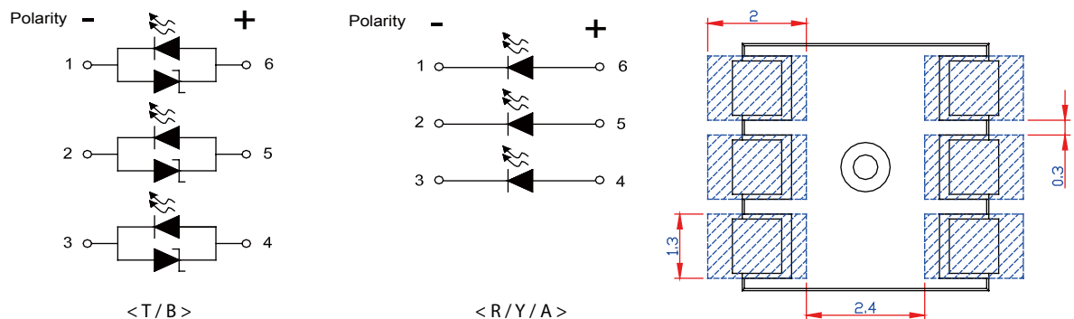
Figure 3. PLCC 5050 series circuit diagram and recommended soldering pad
