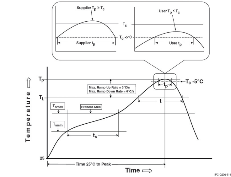
Figure 8. Reflow Profiles
