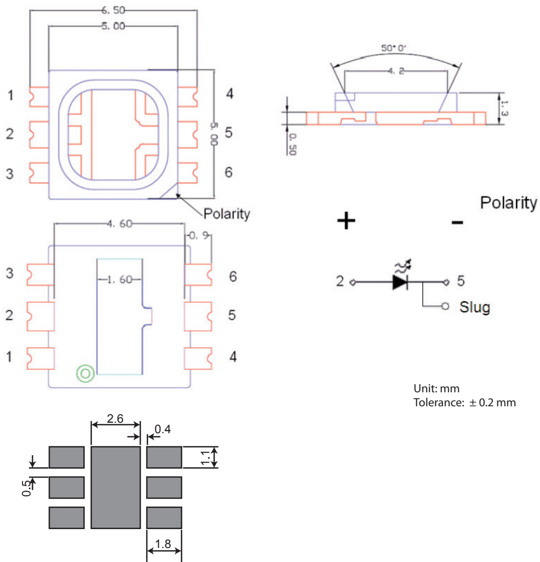
Figure 1. 5050W PLCC Dimension, circuit diagram and recommended soldering pad
