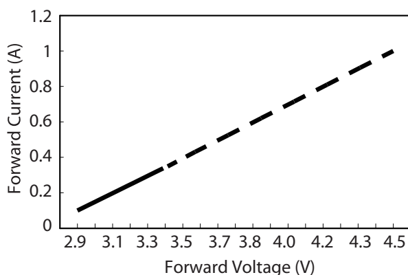
Figure 3. Forward current & forward voltage for 1W PLCC
