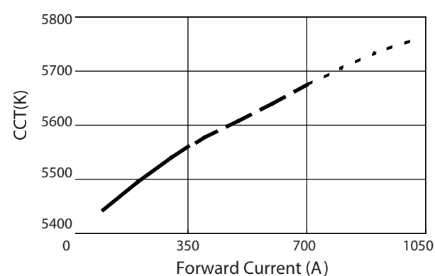
Figure 5. Forward current & CCT at T_a=25^{\circ}\text{C} for 1W PLCC Neutral White
