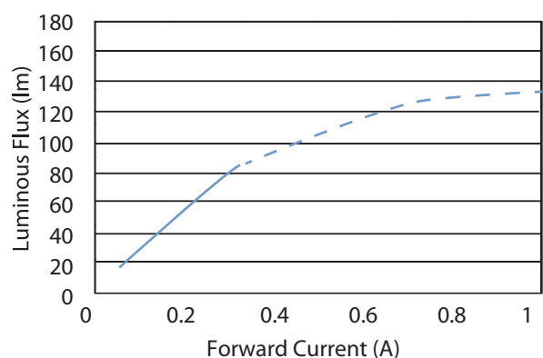
Figure 4. Forward current & relative luminous at T_a=25^{\circ}\text{C} for 1W PLCC
