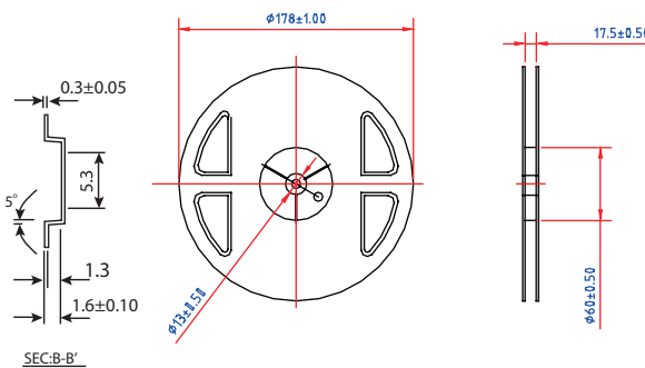
Figure 6. Taping reel dimensions
