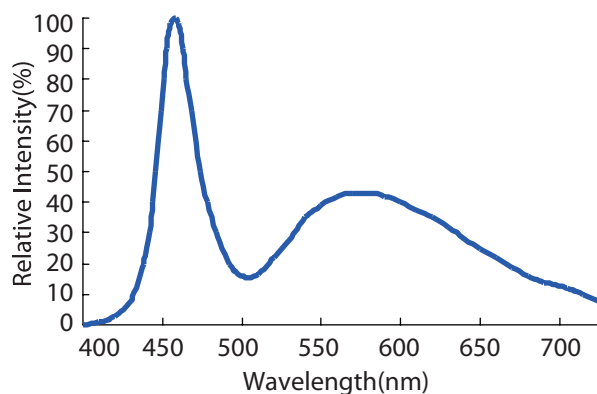
Figure 2. Color Spectrum for Cool White at a typical CCT
