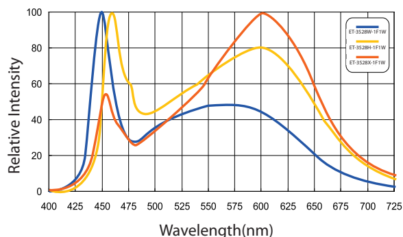
Figure 3. Wavelength & relative intensity for PLCC 5630 series
