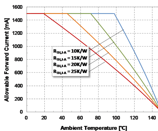
▪ Derating Curve
