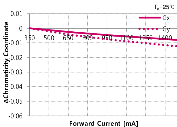
▪ CIE vs. Forward Current
