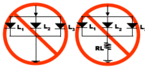
Pic.2 Abnormal Circuit The Current through the LEDs may vary due to the variation in forward voltage ( V_F ) of the LEDs
