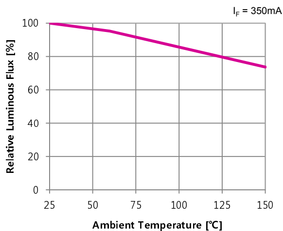
▪ Luminous Flux vs. Ambient Temp.
