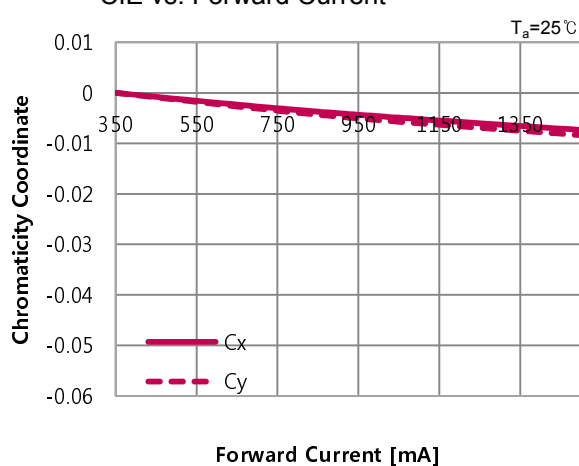
■ CIE vs. Forward Current
