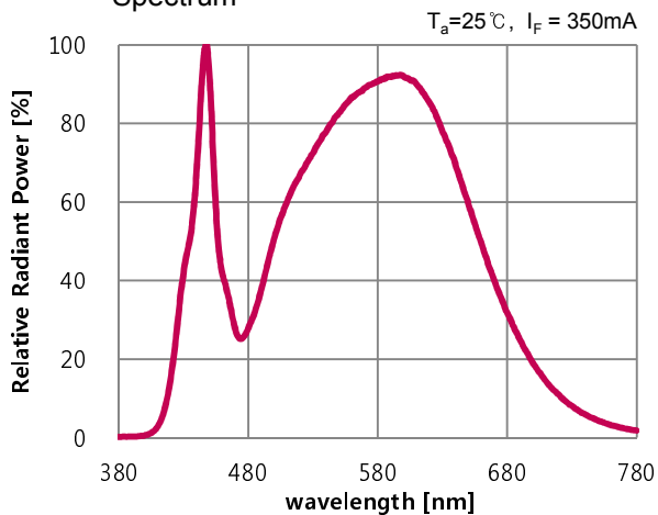
■ Radiation Characteristics
