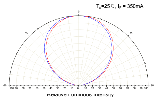
■ Radiation Characteristics
