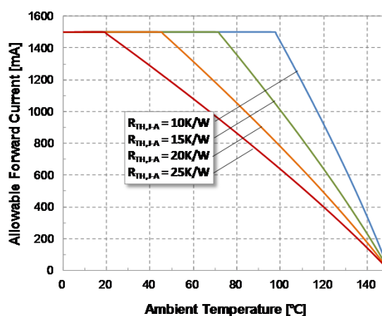
▪ Derating Curve
