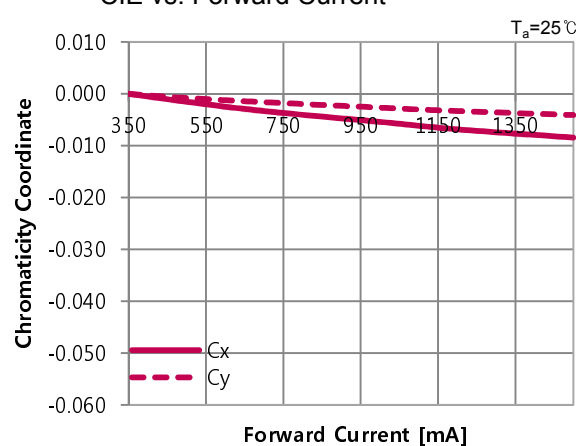
■ CIE vs. Forward Current
