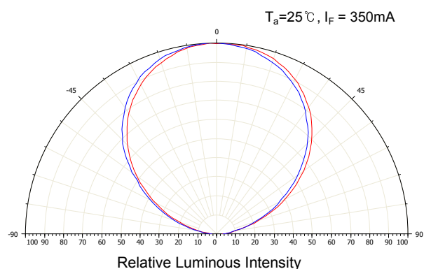
■ Radiation Characteristics
