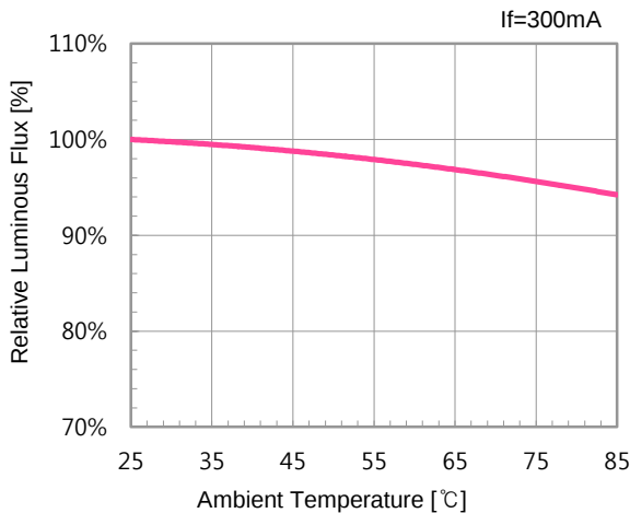
▪ Relative Luminous Flux vs. Temp.
