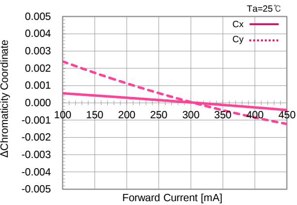
▪ ΔChromaticity Coordinate vs. Forward Current
