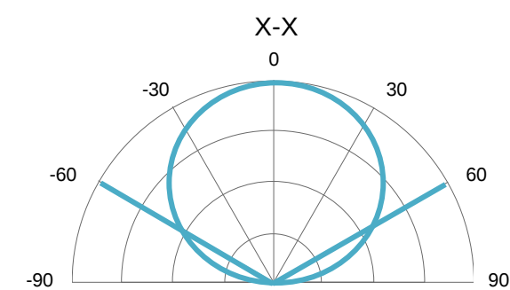
▪ Radiation Characteristics
