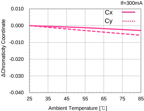
▪ \Delta Chromaticity Coordinate vs. Temp.
