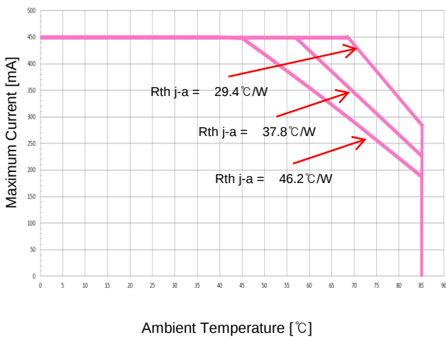
▪ Derating Curve
