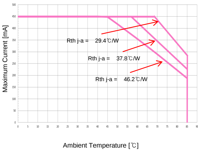
▪ Derating Curve
