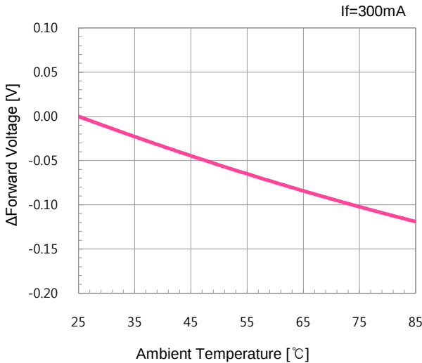
▪ \Delta Forward Voltage vs. Temp.
