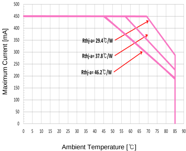
▪ Derating Curve
