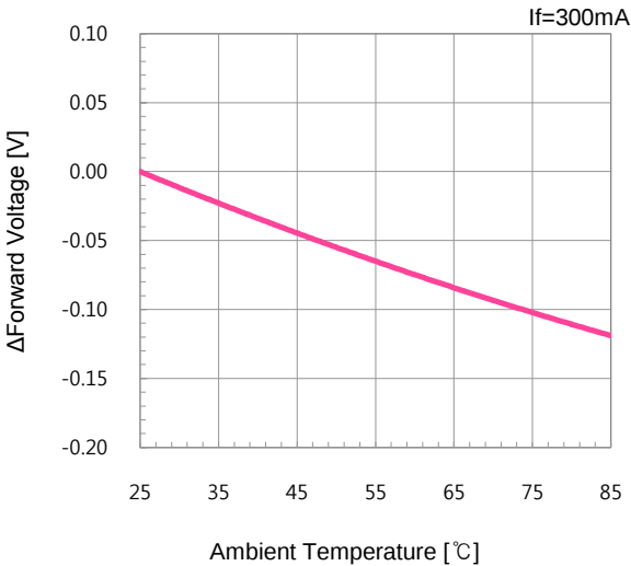
▪ \Delta Forward Voltage vs. Temp.
