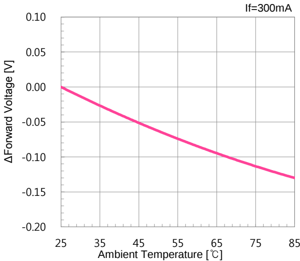
▪ \Delta Forward Voltage vs. Temp.
