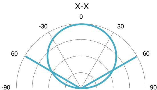
Radiation Characteristics
