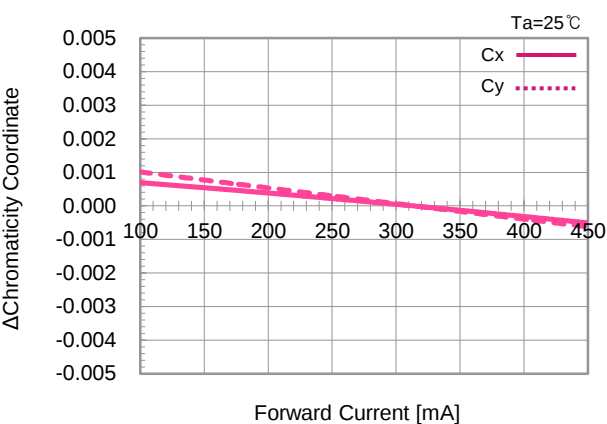
\Delta Chromaticity Coordinate vs. Forward Current
