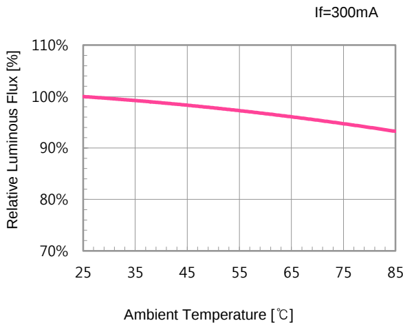
▪ Relative Luminous Flux vs. Temp.
