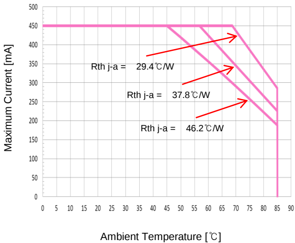
▪ Derating Curve
