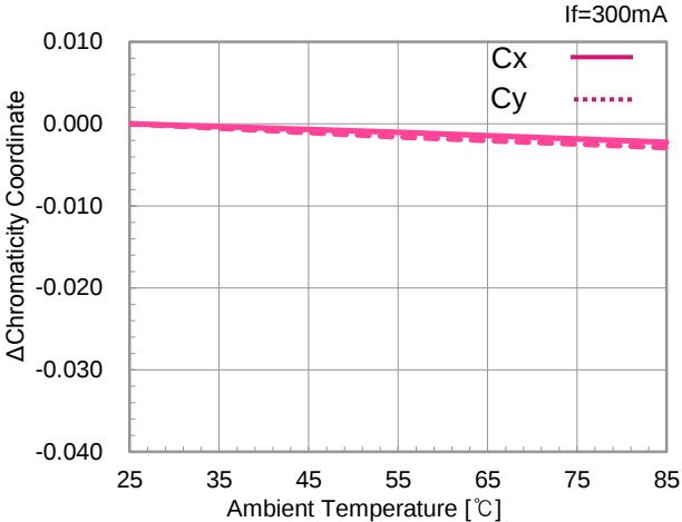
▪ \Delta Chromaticity Coordinate vs. Temp.
