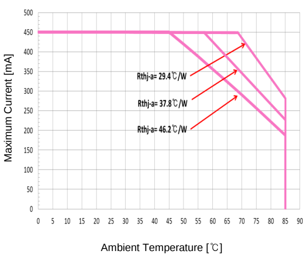
▪ Derating Curve
