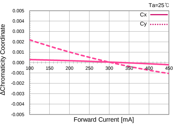
▪ \Delta Chromaticity Coordinate vs. Forward Current
