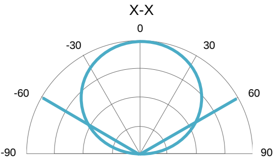
▪ Radiation Characteristics
