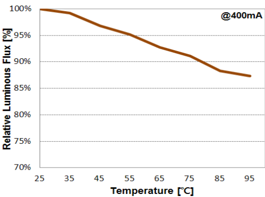
■ Luminous Flux vs. Temp.
