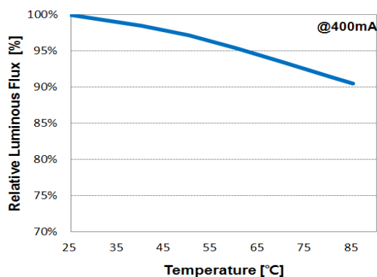
■ Luminous Flux vs. Temp.
