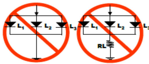
Pic.2. Abnormal Circuit The Current through the LEDs may vary due to the variation in forward voltage ( V_f ) of the LEDs.
