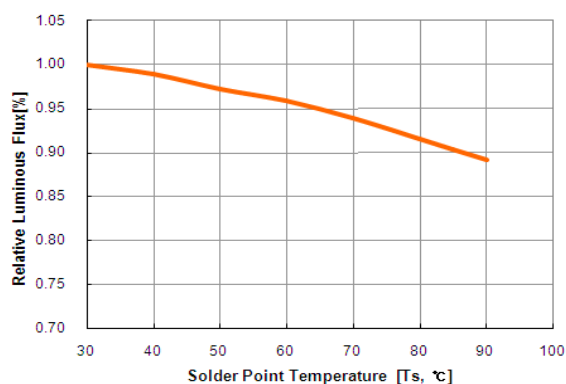
■ Luminous Flux Vs TEMP.
