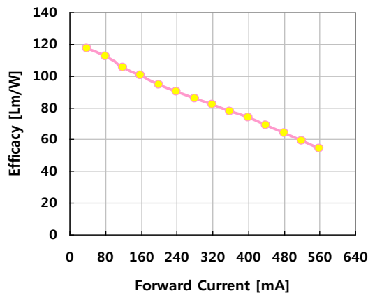
■ Input Watt vs. Luminance Flux
