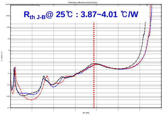
■ Thermal Resistance (junction~Board)
