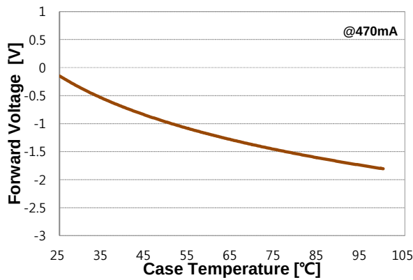
■ ΔForward Voltage vs. Temp.
